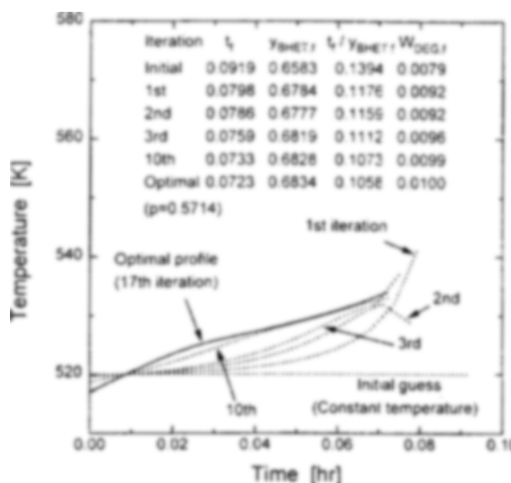
Fig. 2. An example showing how the reactor temperature profile can be improved by the iteration based on the gradient of the Hamiltonian.
